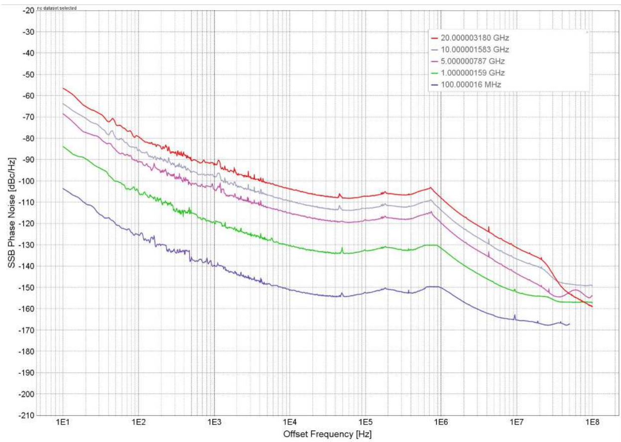
Figure 2. Phase noise performance
