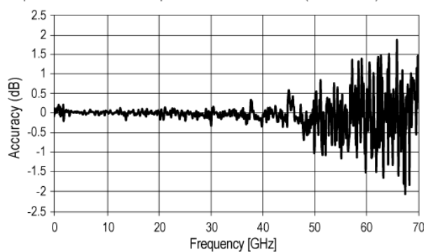
Option 521 level accuracy at +24 dBm (measured)
