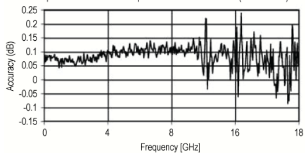
Option 532/540 with Option 1E1 at -110 dBm (measured)
