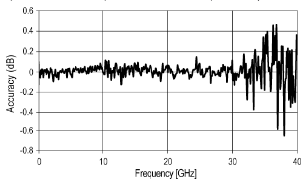
Option 521 level accuracy at -110 dBm (measured)
