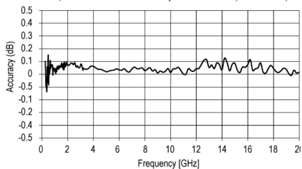
Option 521 level accuracy at +24 dBm (measured)
