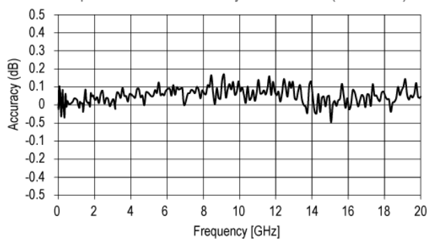
Option 521 level accuracy at -110 dBm (measured)
