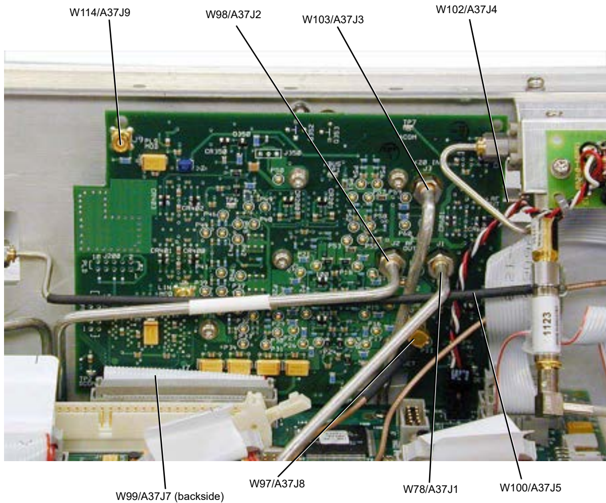
Figure 3-65 A37 Upconverter
