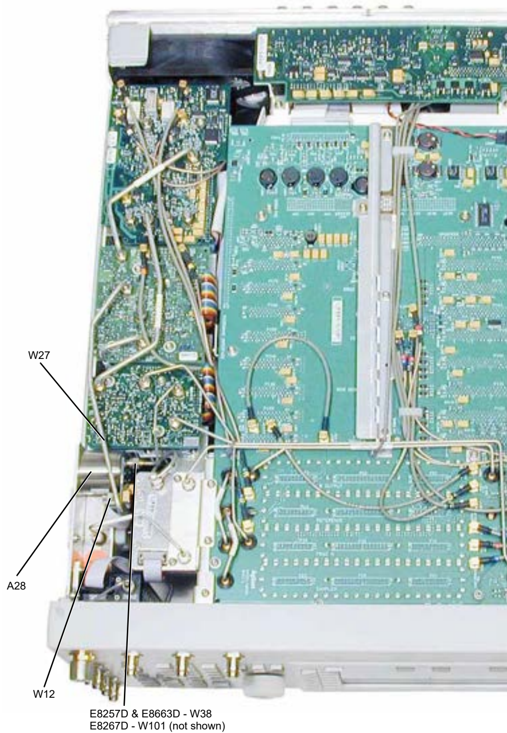
A28 YIG Oscillator
