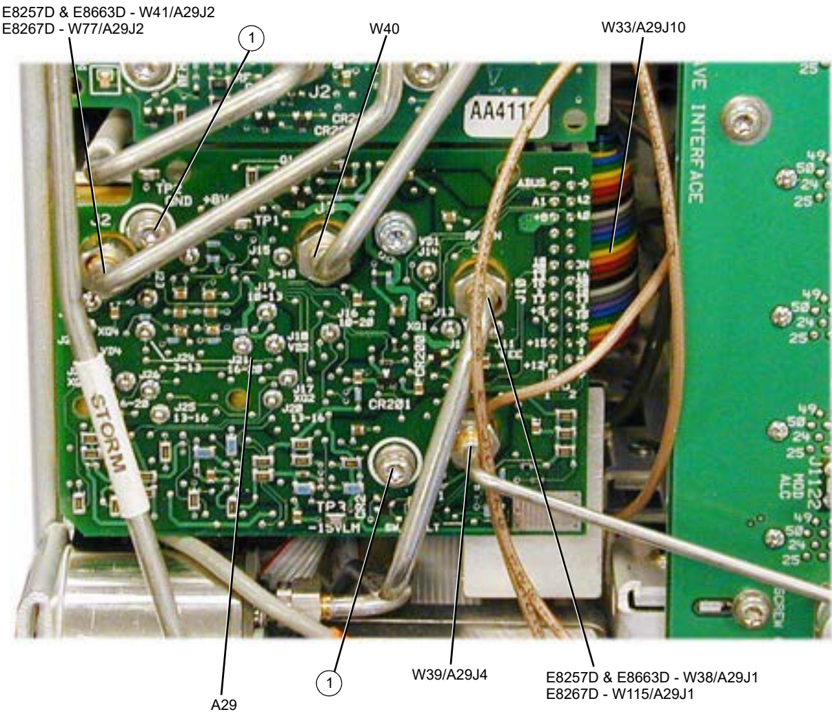
Figure 3-52 A29 20 GHz Doubler
