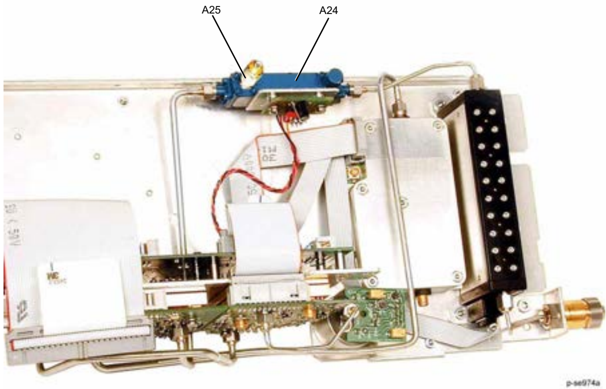
Figure 3-43 A25 40 GHz Highband Detector (Option 540)
