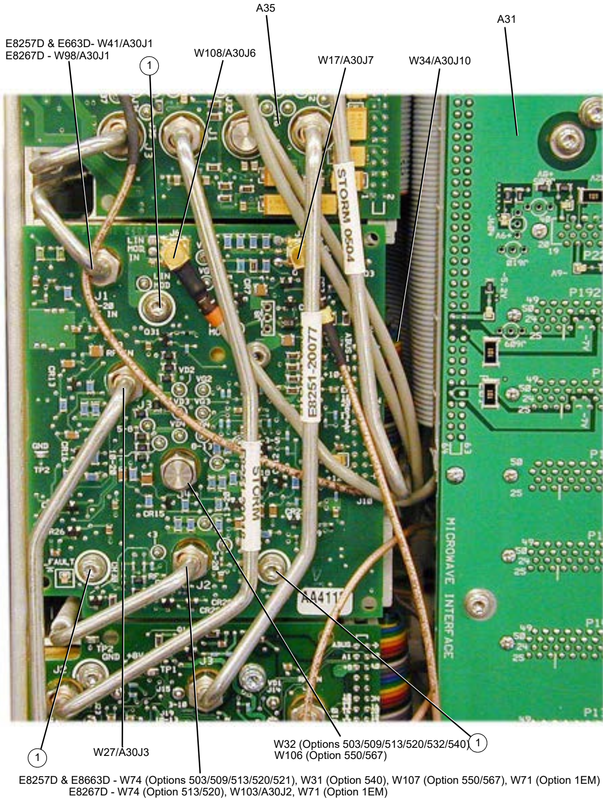
Figure 3-53 A30 Modulator Filter
