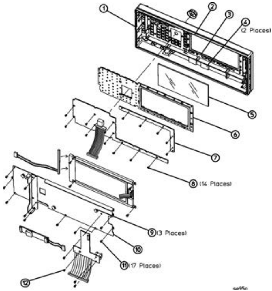
Figure 2-17 Disassembled Front Panel View
