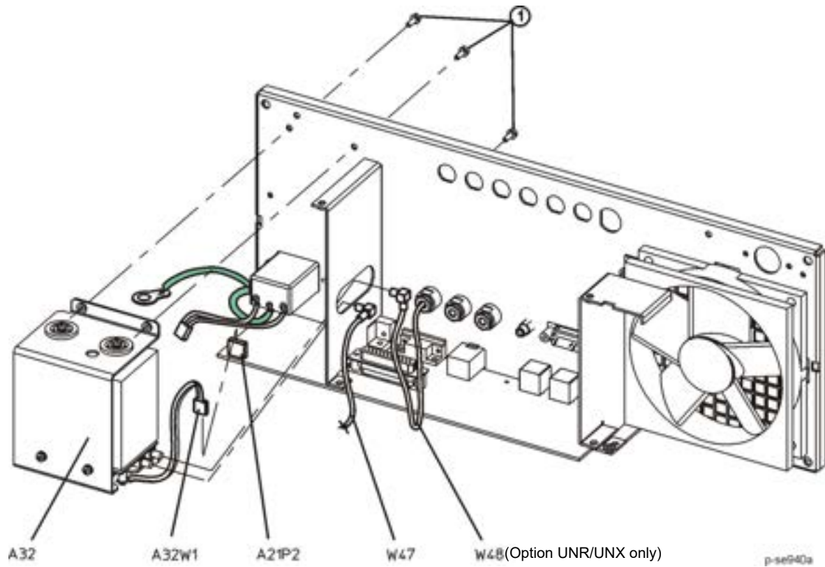
Figure 3-56 A32 Crystal Oscillator
