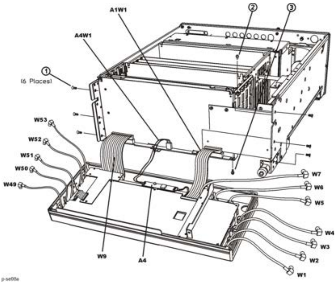
Figure 3-3 Front Panel Removal with serial prefixes < US/MY5XXX3XXX 1
