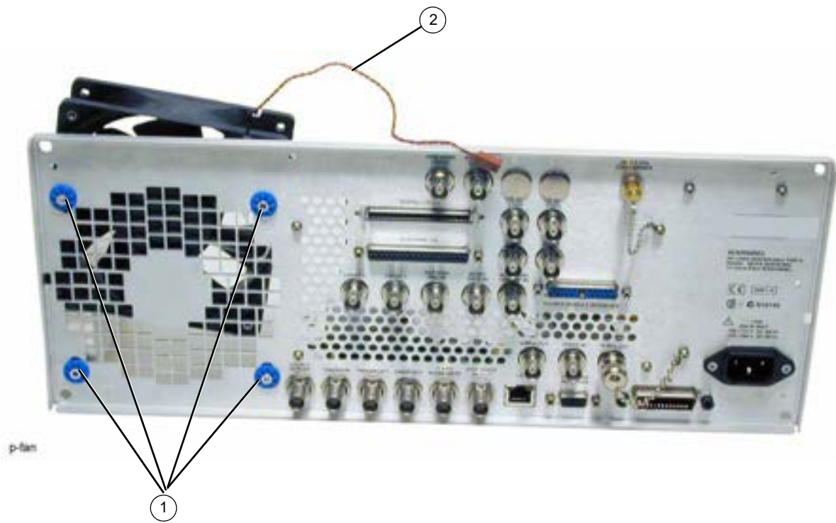
Figure 3-78 B1 Fan
