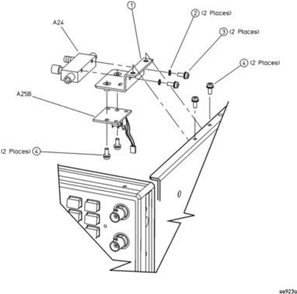
Figure 2-22 Disassembled A24 20GHz/40GHz Highband Coupler and A25B Highband Detector Bias Board
