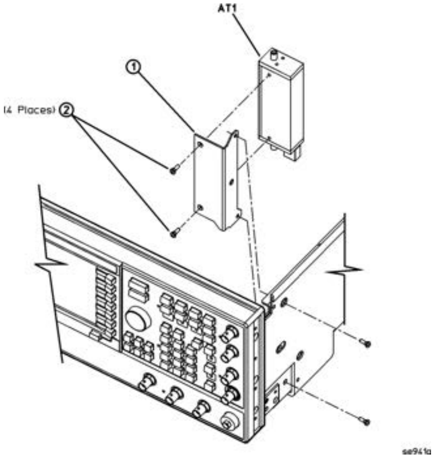
Figure 2-21 Disassembled AT1 90dB/115dB Attenuator View (Option 1E1)
