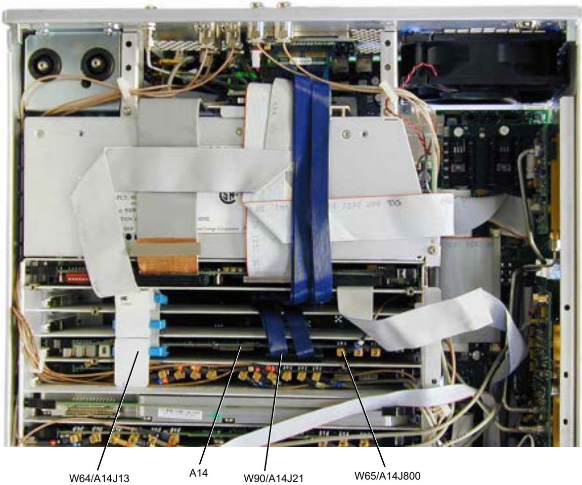
Figure 3-22 A14 Baseband Generator
