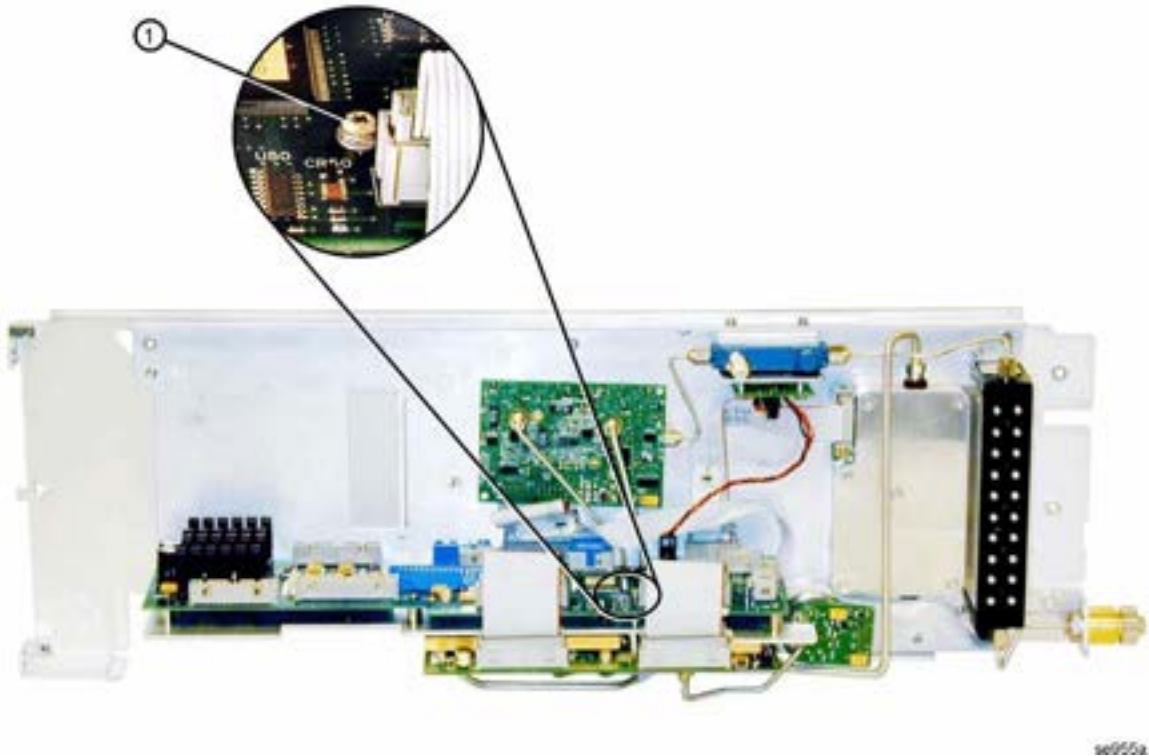
Figure 2-27 E8267D Microcircuit Interface Deck Top View
