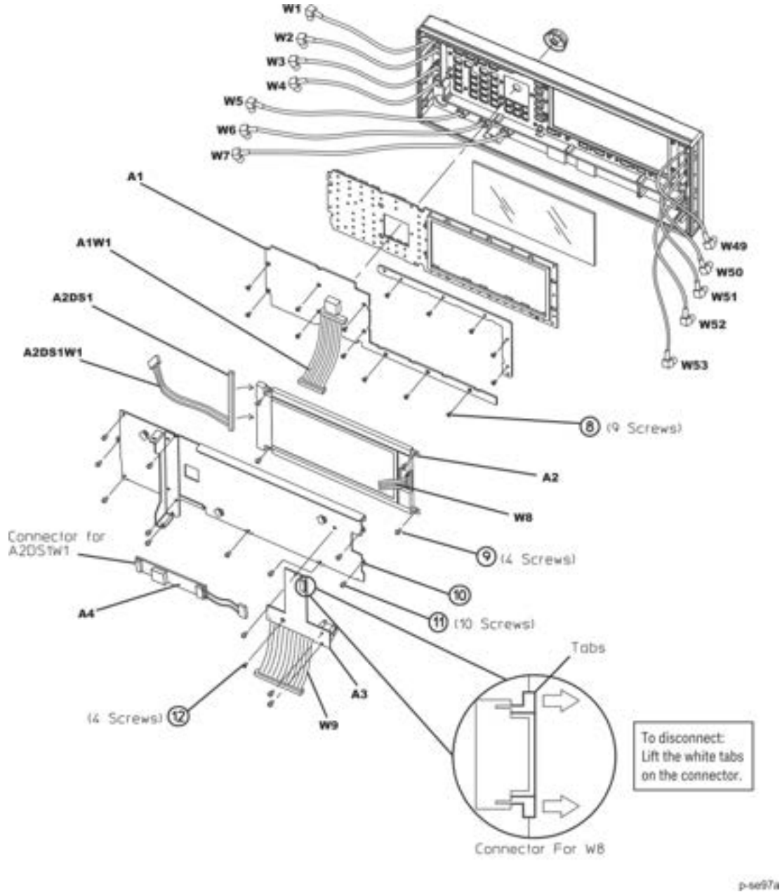
Figure 3-10 A3 Power Switch Removal with serial number prefix < US/MY5XXX3XXX 1
