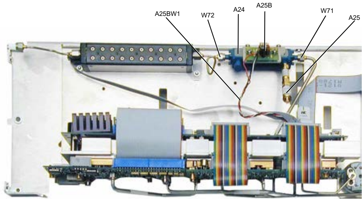
Figure 3-36 A24 40 GHz Highband Coupler (Option 540 - Option 1EM)
