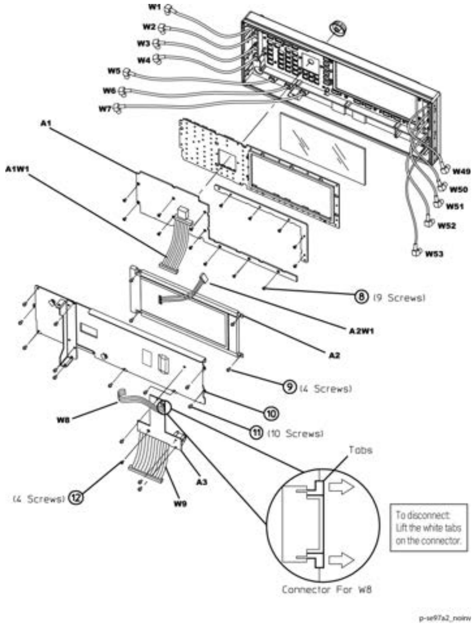
Figure 3-8 A2 Display Removal with serial prefixes \geq US/MY5XXX3XXX
