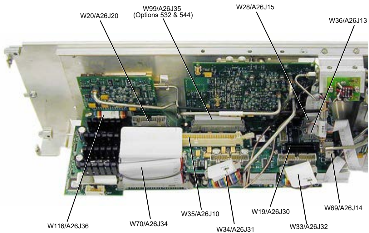
Figure 3-48 A26 MID (E8267D)
