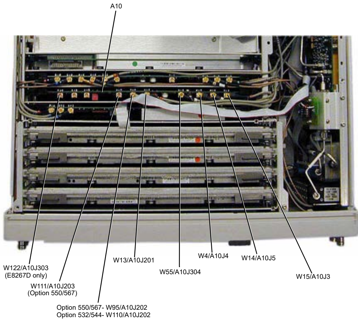
Figure 3-17 A10 ALC
