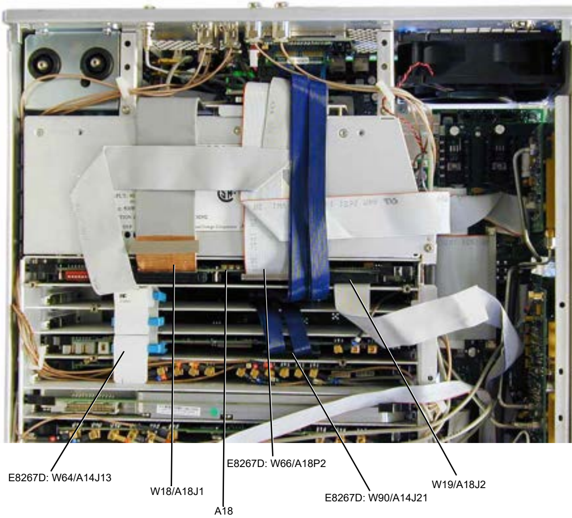
Figure 3-24 A18 CPU
