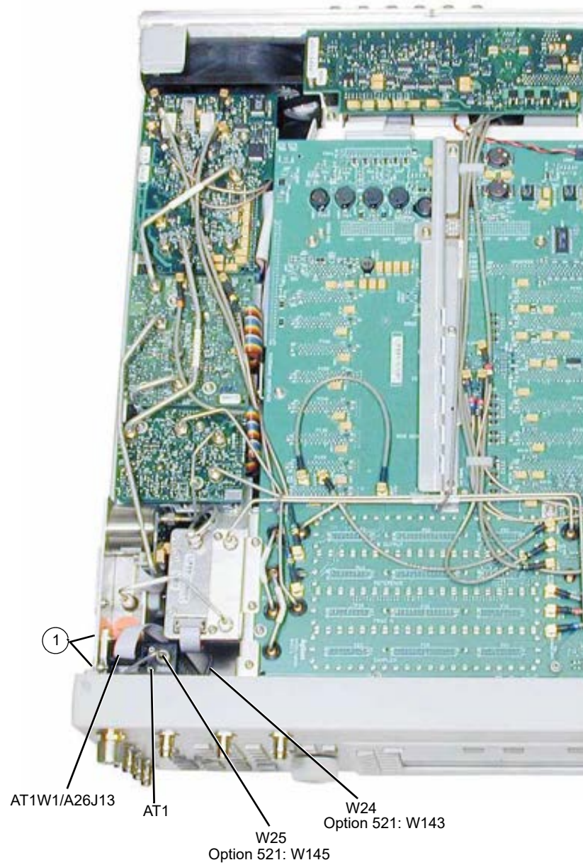
Figure 3-75 AT1 115 dB Attenuator
