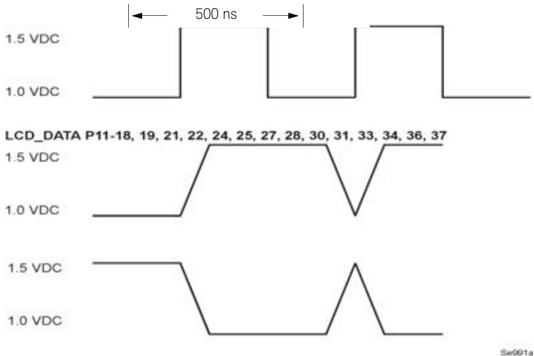
Figure 1-1 Pulsing Activity LCD_CLK P11-9, P221-50
