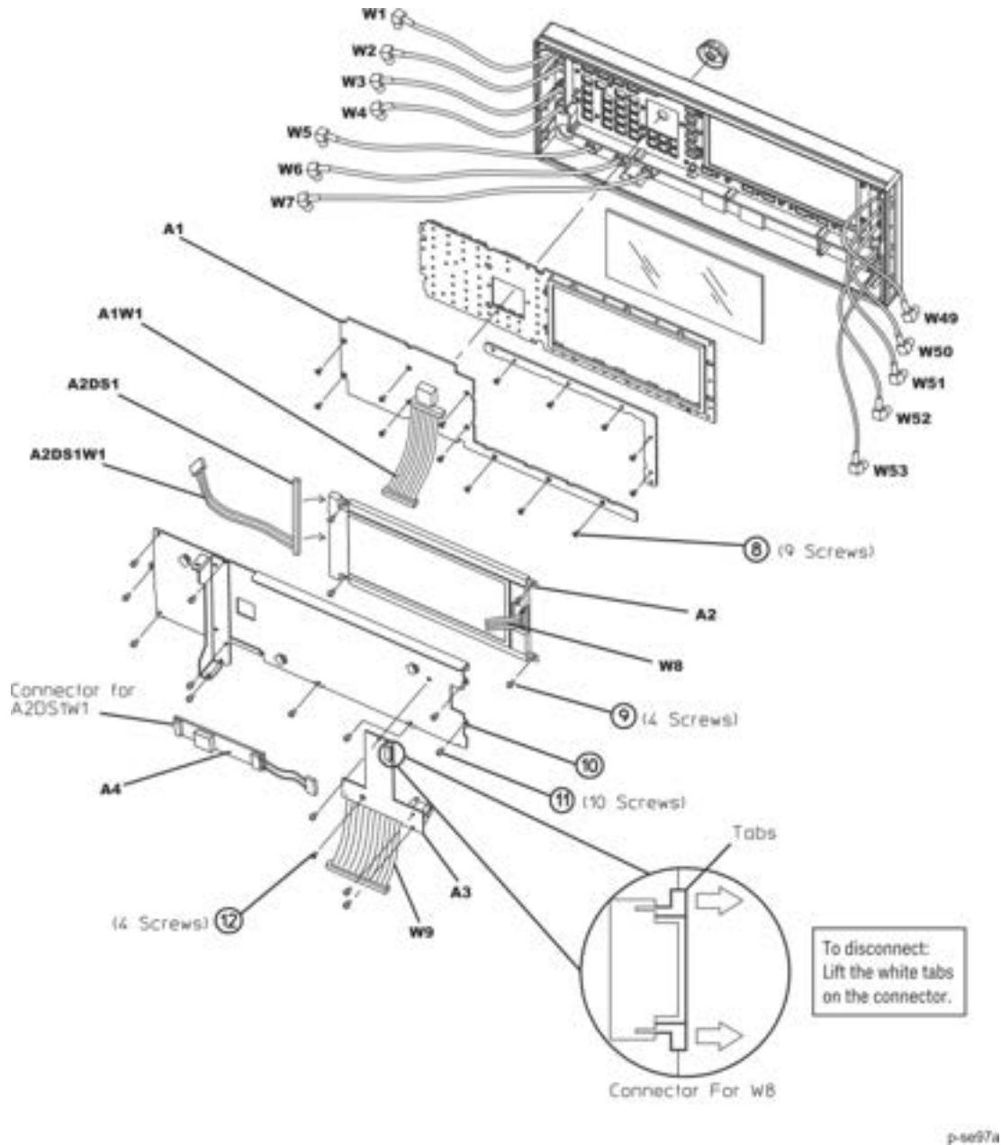
Figure 3-7 A2 Display Removal with serial prefixes < US/MY5XXX3XXX 1
