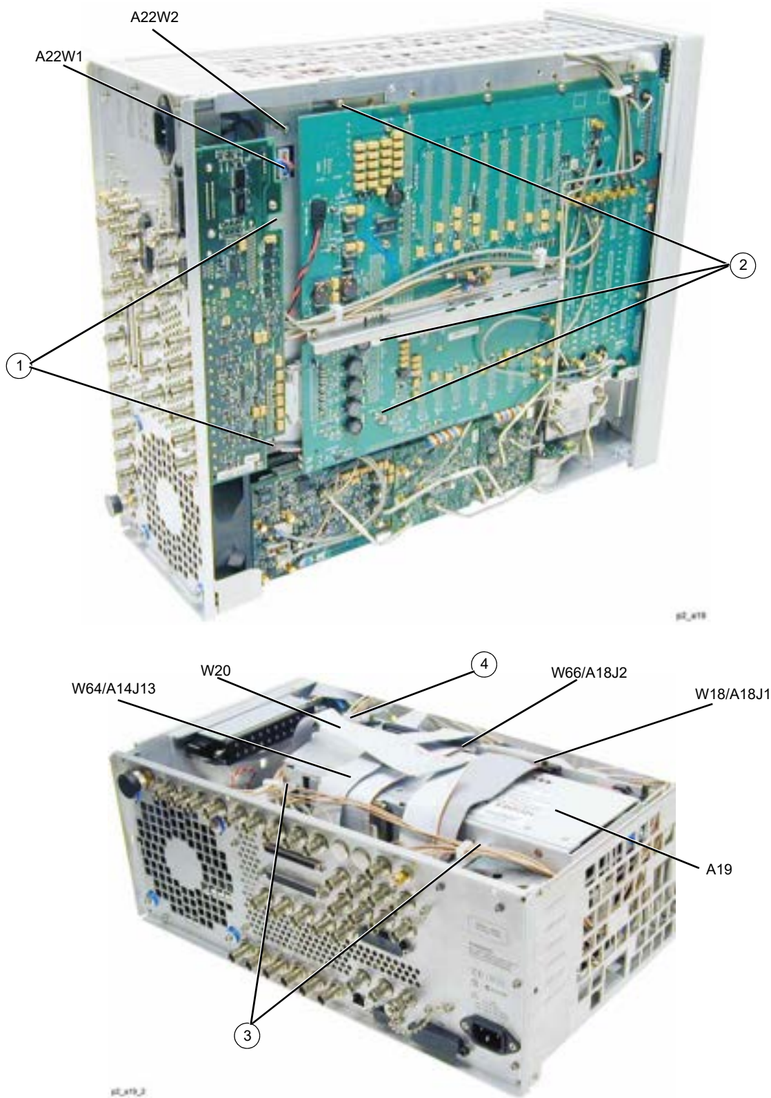
Figure 3-26 A19 Power Supply Removal
