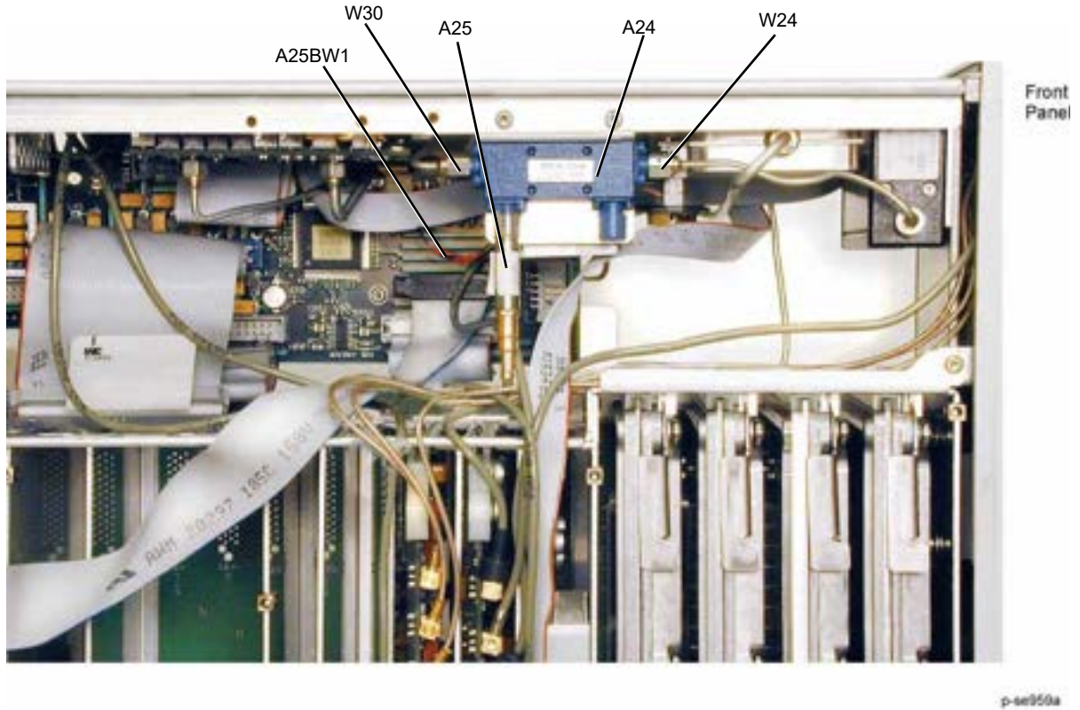
Figure 3-35 A24 40 GHz Highband Coupler (Option 540 - Standard)
