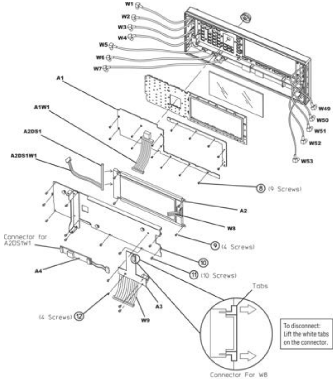
Figure 3-5 A1 Keyboard Removal with serial prefixes < US/MY5XXX3XXX 1
