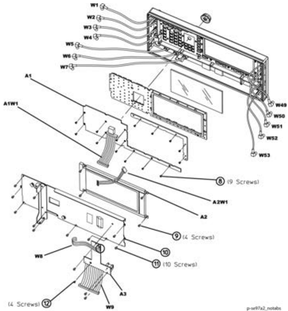
Figure 3-12 A3 Power Switch Removal with serial number prefix \geq MY6136XXXX
