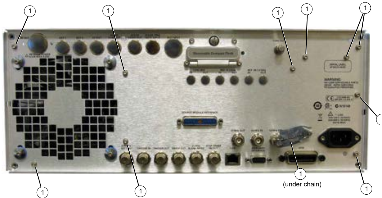
Figure 3-59 Rear Panel Removal
