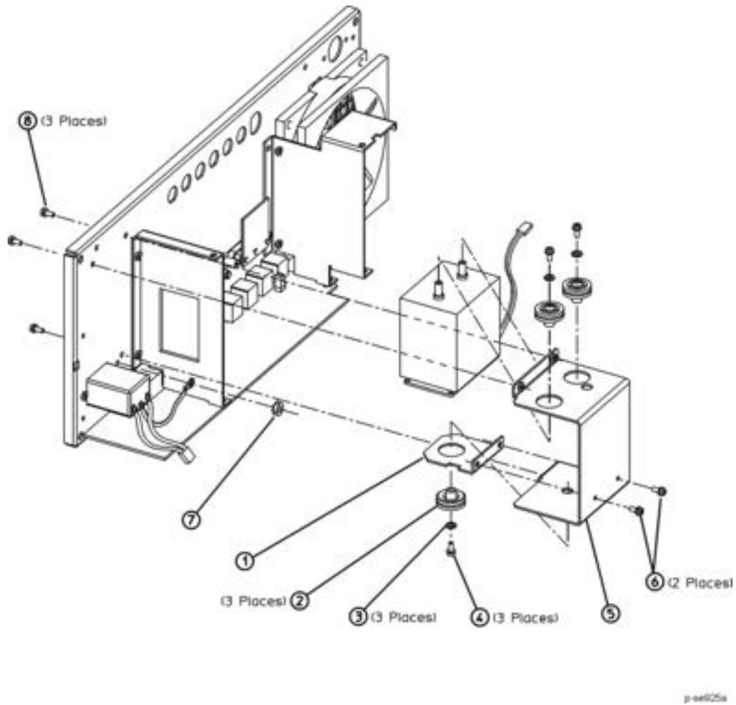
Figure 2-20 Disassembled A32 10 MHz Crystal Oscillator (Option UNR/UNIX and Instruments with Serial Prefixes \geq US4805/MY4805)
