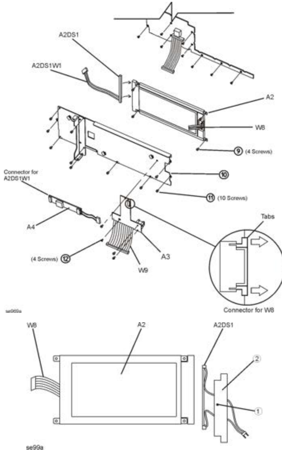
Figure 3-9 A2DS1 Display Backlight Removal
