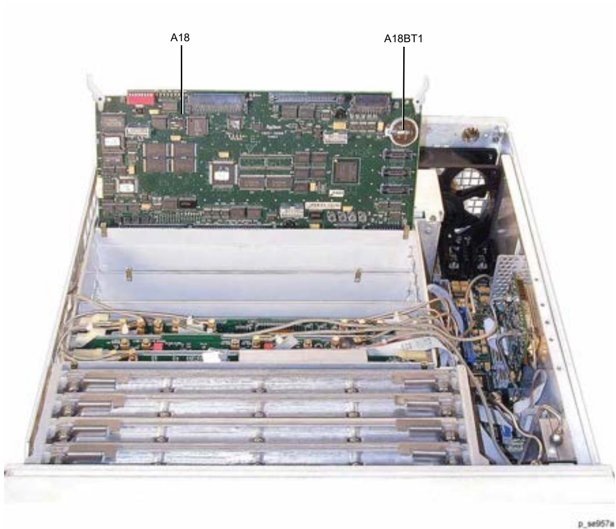
Figure 2-15 A18BT1 Lithium Battery
