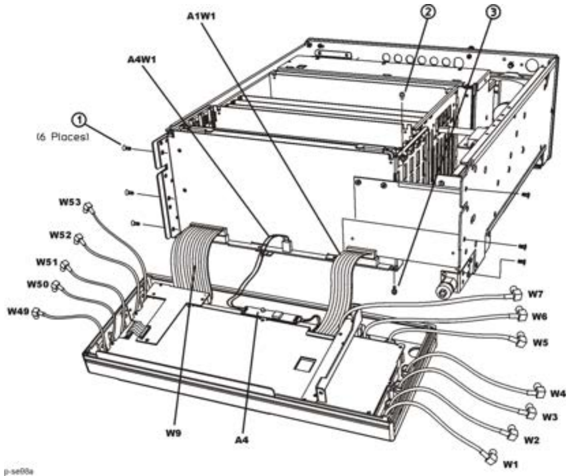
Figure 3-13 A4 Inverter Removal
