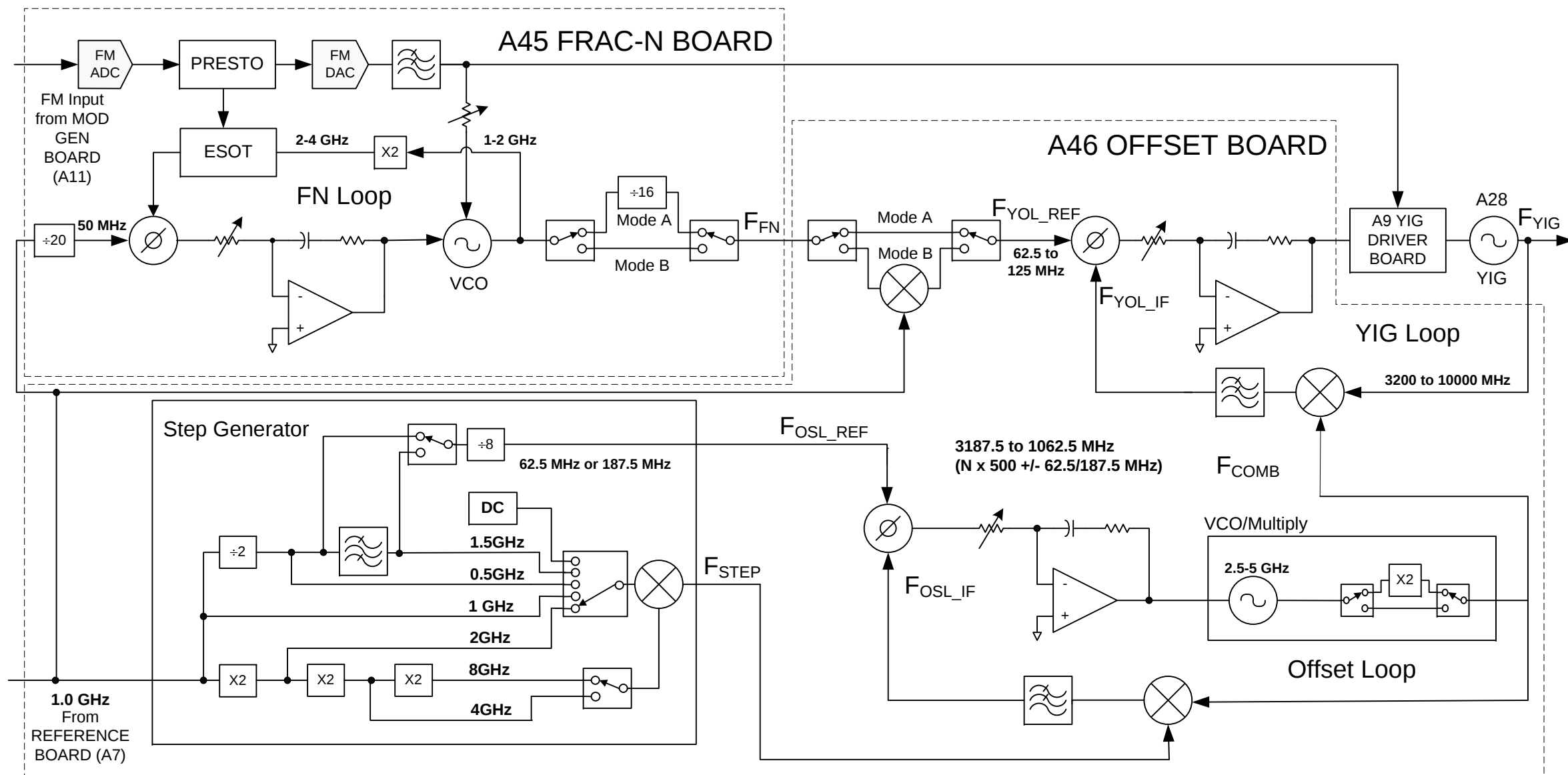
Block Diagram for Option UNY, Service Guide E8251-90359 (prefix ≥US5042/MY5042/SG5042)
