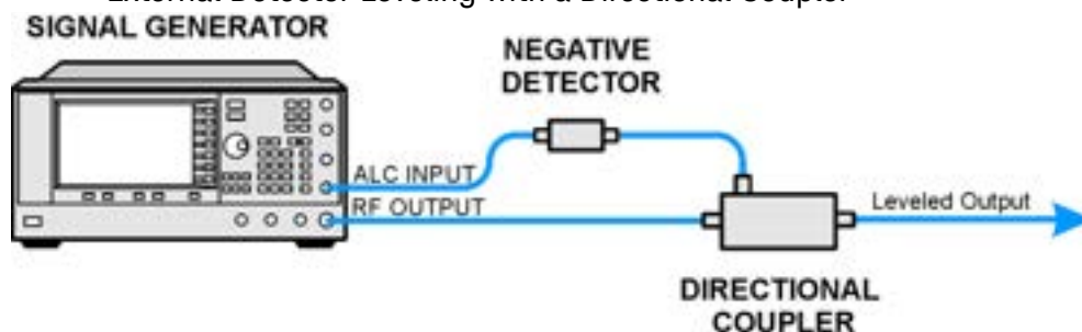
Figure 4-2 External Detector Leveling with a Directional Coupler
