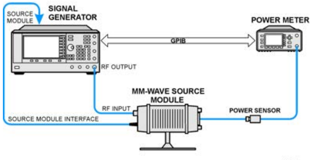
Figure 4-6 User Flatness with mm-Wave Source Module for Signal Generators with Options 1EA, 1EU, or 521
