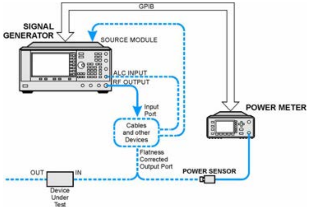
User Flatness Correction Equipment Setup
