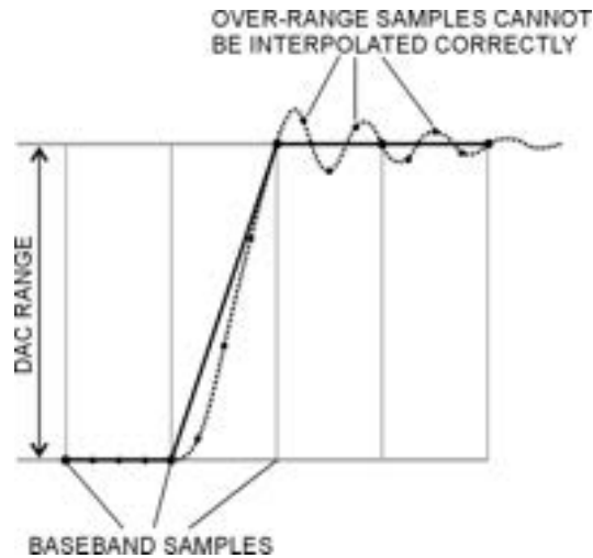
Figure 3-18 Waveform Overshoot
