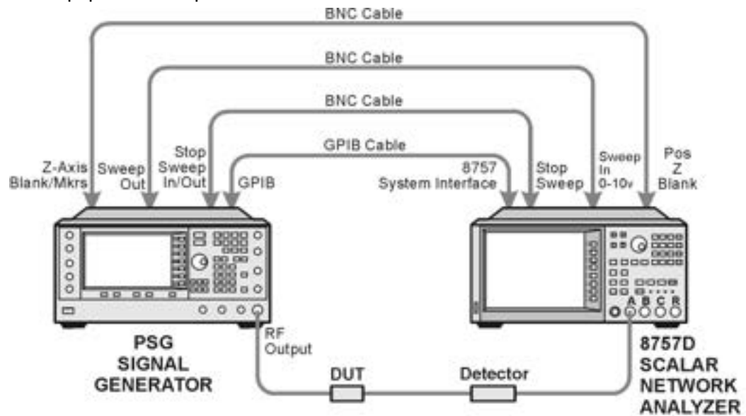
Figure 2-3 Equipment Setup
