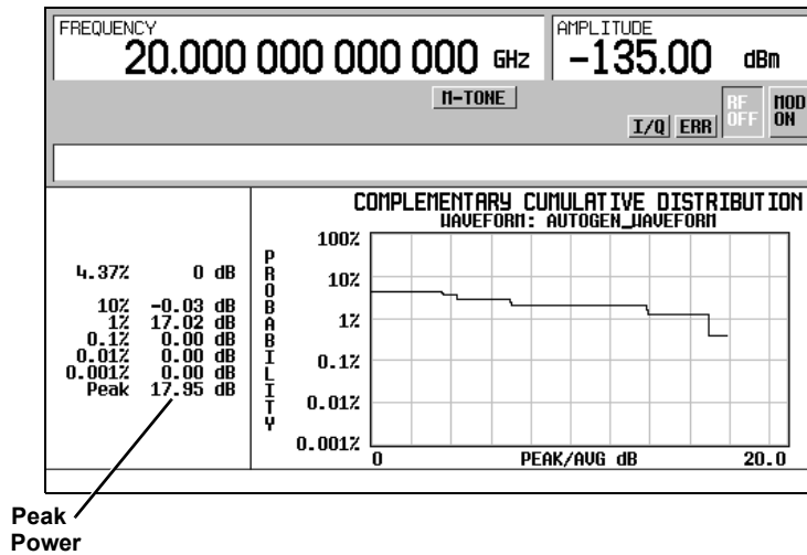
Figure 9-7 CCDF Plot with Fixed Phase Set
