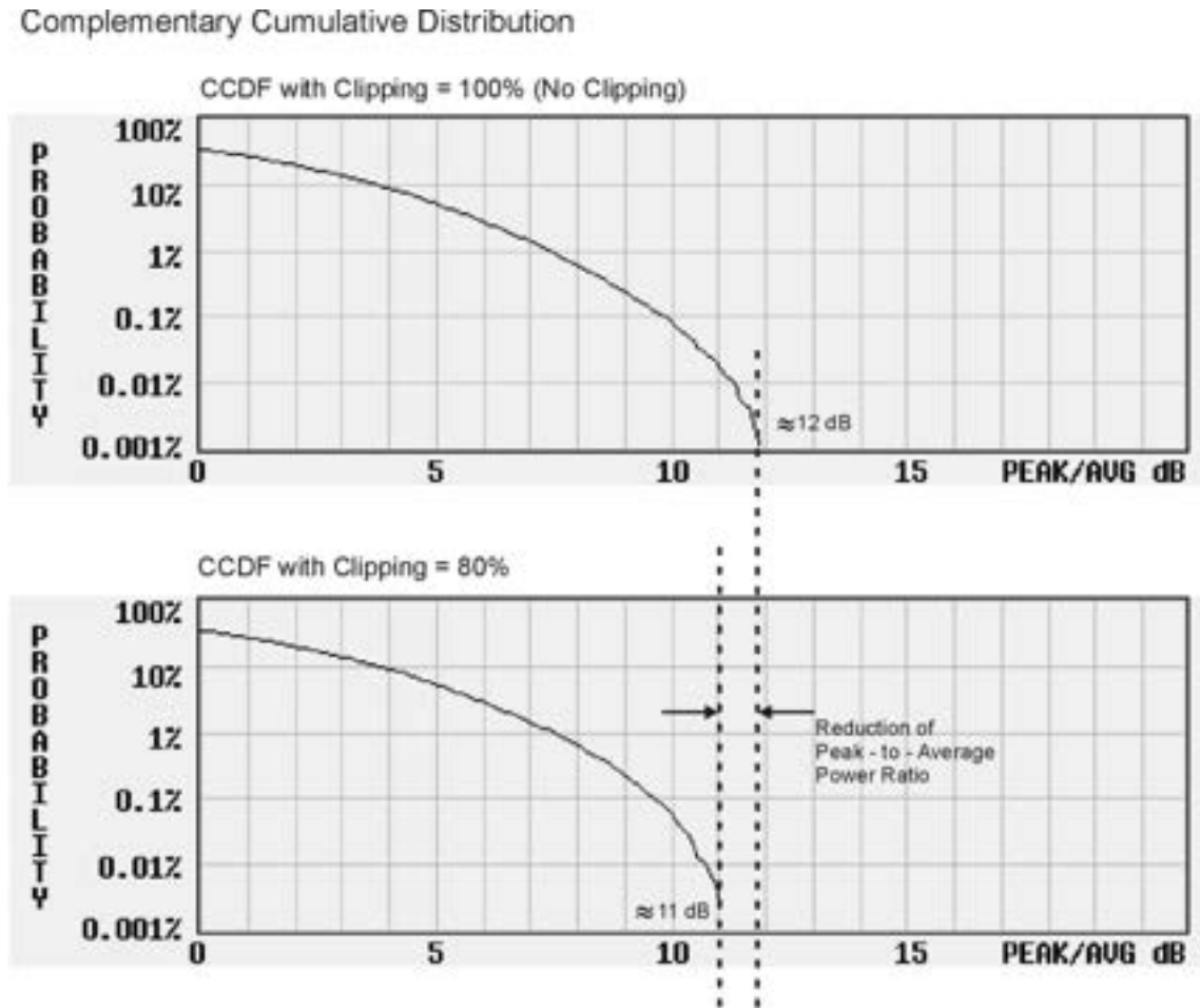
Figure 3-16 Reduction of Peak-to-Average Power
