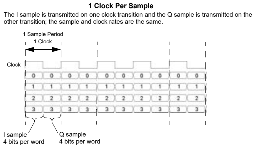
Clock Timing for a Parallel IQ Interleaved Port Configuration
