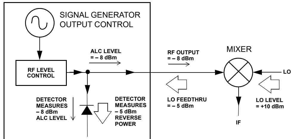
Effects of Reverse Power on ALC
