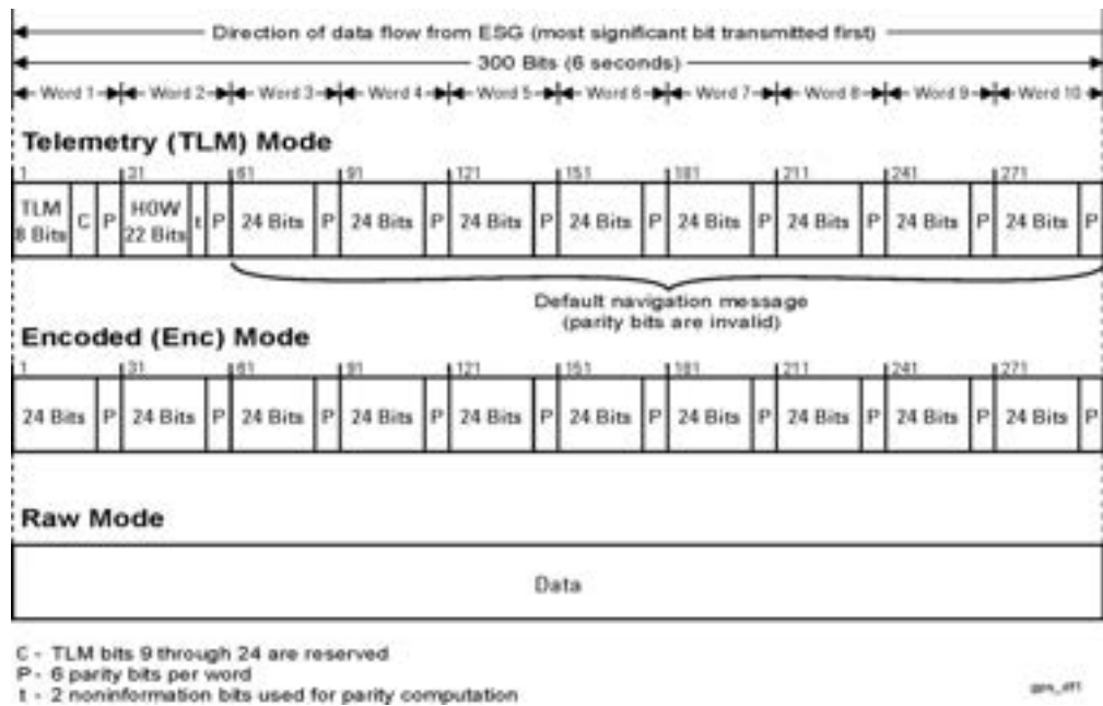
Figure 8-4 Subframe Structures
