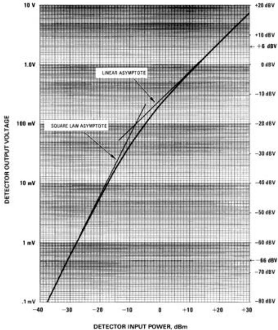
Typical Diode Detector Response at 25° C
