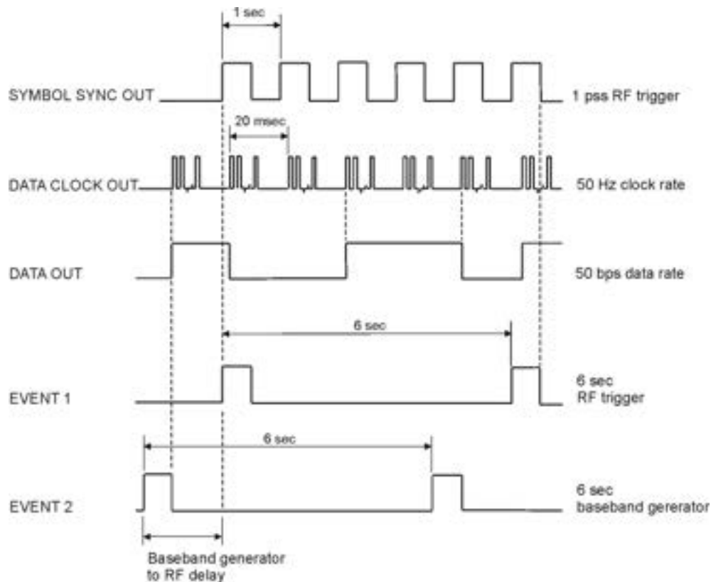
GPS Signals
