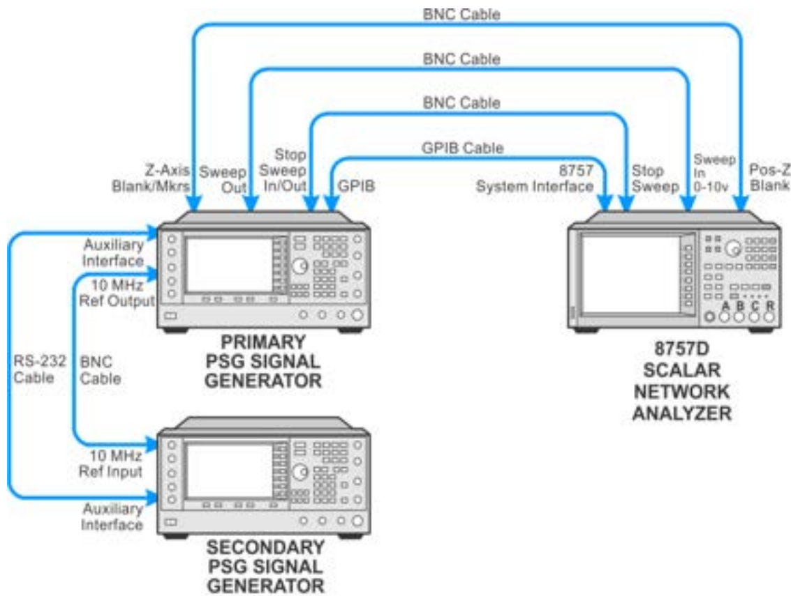
Figure 2-8 Primary/Secondary Equipment Setup
